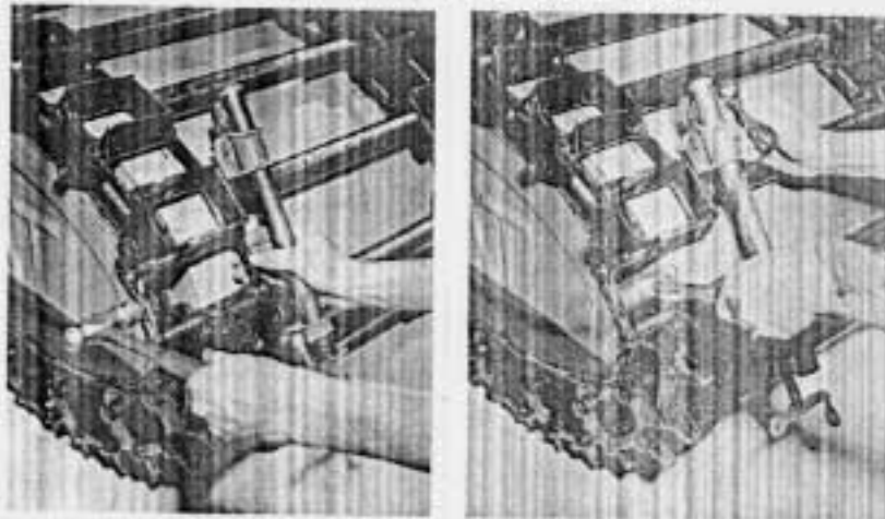
COUPLE OR UNCOUPLE TRACK WITH CLAMP
